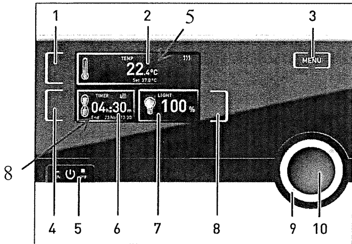
Fig. 13 ControlCOCKPIT of Peltier-cooled incubators IPP in operating mode
